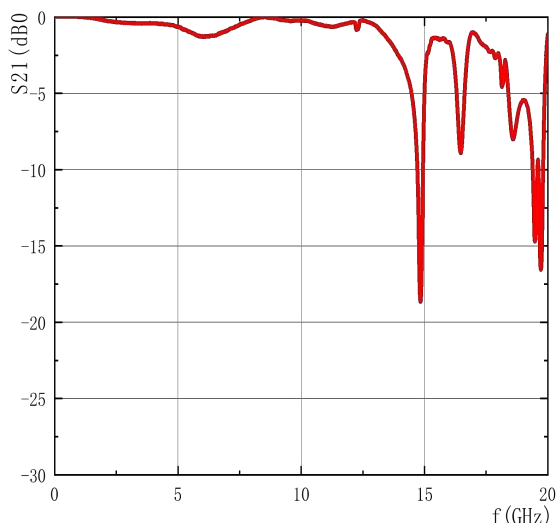
插入损耗 Insertion Loss S21 (标识代号 identification code: IL-BNC-A)
